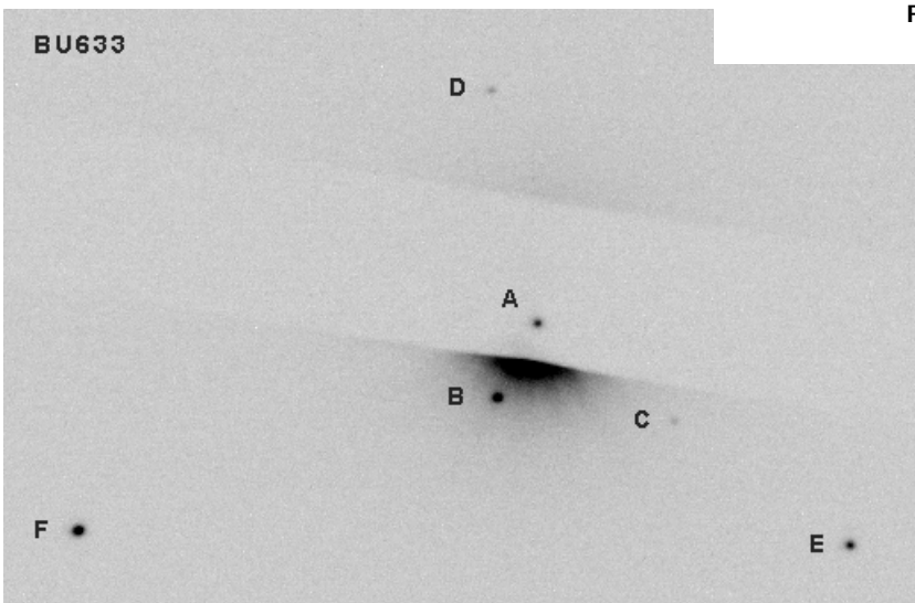
Figure 6: Gamma Draco, 10 sec exp, no binning, cropped.
